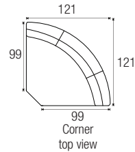
99 Corner top view
